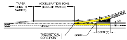
PARTIAL LIGHTING PARALLEL ON-RAMP ACCELERATION LANE
