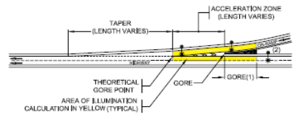
PARTIAL LIGHTING SINGLE LANE ON-RAMP WITH TAPER
