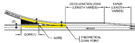
PARTIAL LIGHTING PARALLEL OFF-RAMP DECELERATION LANE
