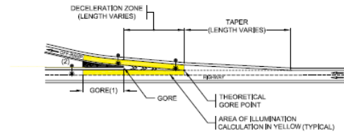
PARTIAL LIGHTING SINGLE LANE OFF-RAMP WITH TAPER
